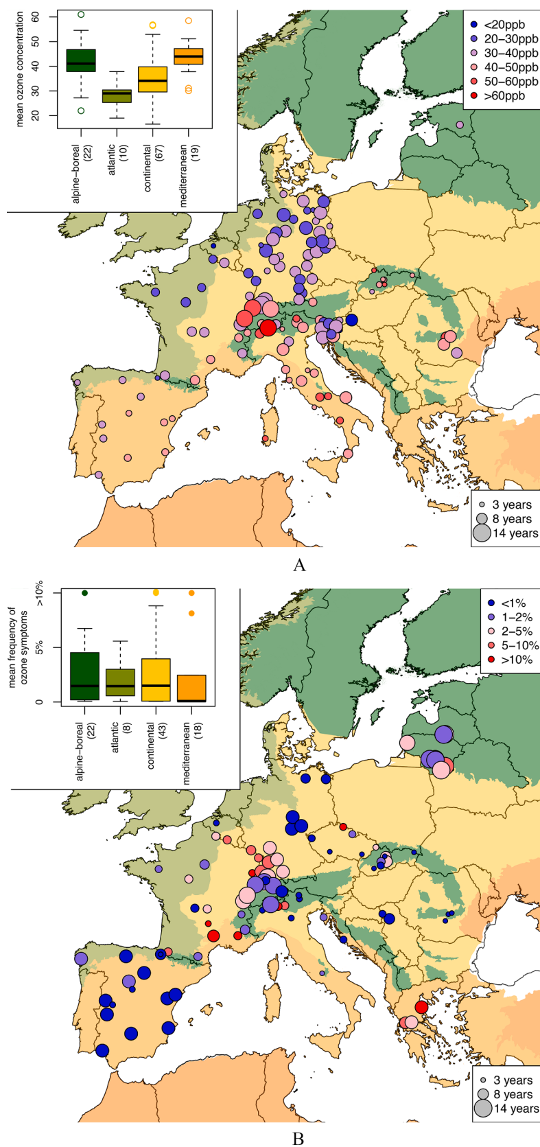
Fig. 3. Mean April-September concentrations of ozone (A, 118 sites) and mean frequency of VFS (B, 91 sites) across different biogeographic regions (inset boxplots diagrams) in Europe from 2005 to 2018. The size of the dots on the maps indicates the number of years with data availability for each plot (from 3 to 14). The upper-left boxplot indicates the variation among biogeographic regions and the color keys to the map. The number of plots per biogeographic region is indicated in brackets.
