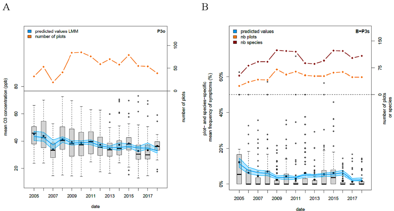
Fig. 5. Temporal changes in ozone concentrations and VFS. Temporal change in (A) ozone mean April–September concentrations (P30 subset) and (B) in frequency of VFS for the plots with at least 3 years of data (P3S subset). Medians, quartiles, and individual plots are indicated with boxplots; mean values are represented with the black full dots. The mean values predicted by the GLMM1 (A) and GLMM2 (B) and their 95 % confidence intervals (from bootstrapping procedures; n = 100 ) are indicated with the blue curve and polygon. Sample size in terms of the number of plots and species considered are indicated in the upper diagram.
