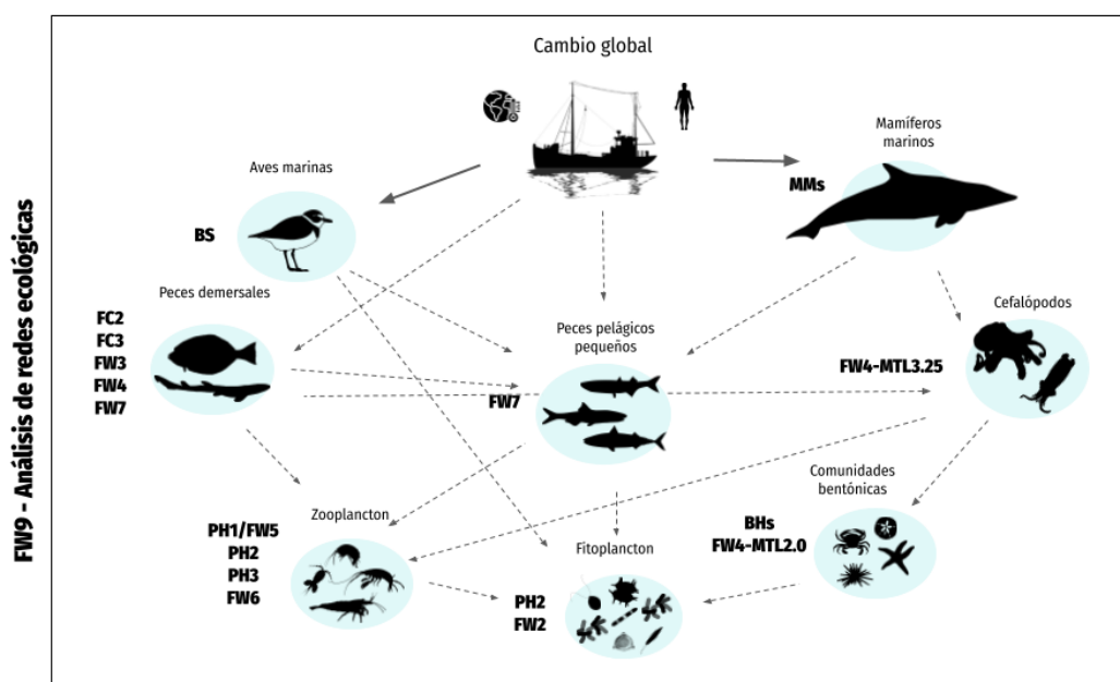
Figura 16. Esquema ilustrativo del indicador RT-ENA (Análisis de Redes Ecológicas) mostrando los vínculos entre los diferentes indicadores, descriptores y componentes del ecosistema. Acrónimos utilizados en OSPAR: BS = seabird breeding success; FC2 = Proportion of Large Fish; FC3 = Mean maximum length of demersal fish and elasmobranchs; FW3 = Size composition in fish communities; FW4 = Changes in Average Trophic Level of Marine Consumers; FW7 = Biomass and abundance of fish functional groups; PH1/FW5 = Change in plankton; PH2 = Plankton biomass and/or abundance; PH3 = Plankton Diversity Index; FW6 = Biomass, species composition, and spatial distribution of zooplankton; FW2 = Production of phytoplankton; MTL = Mean Trophic Level; MMs = Marine Mammals.
