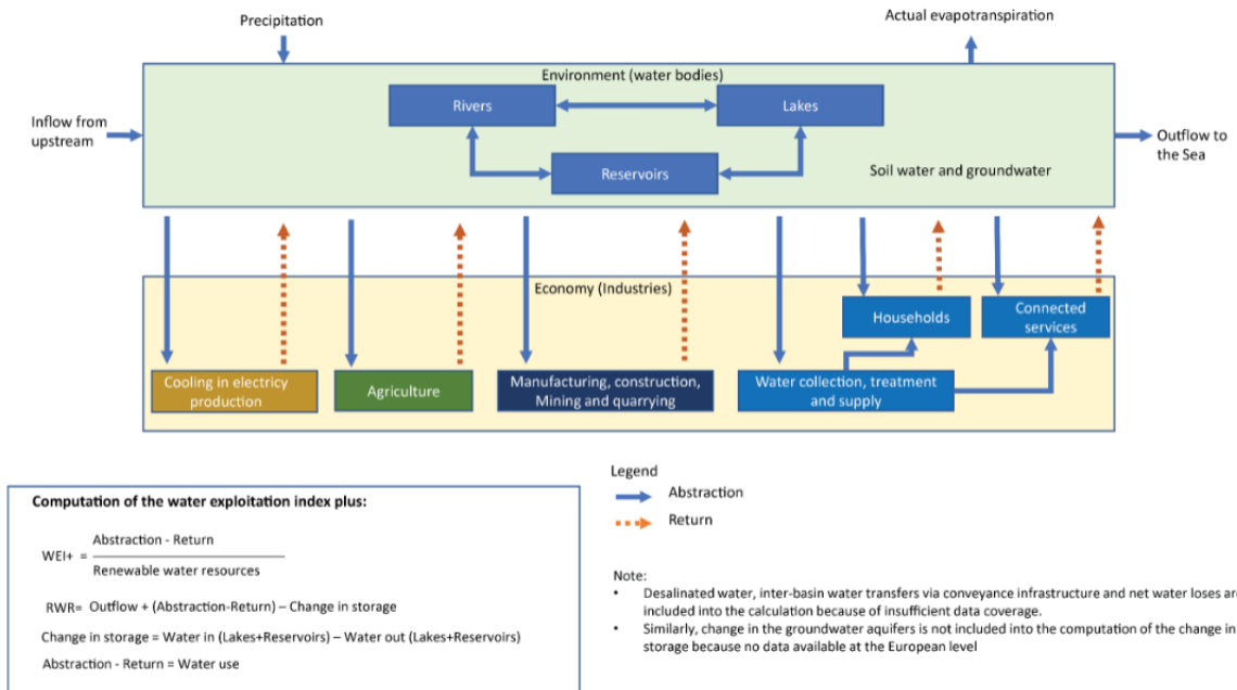
Conceptual model of the WEI+ computation
