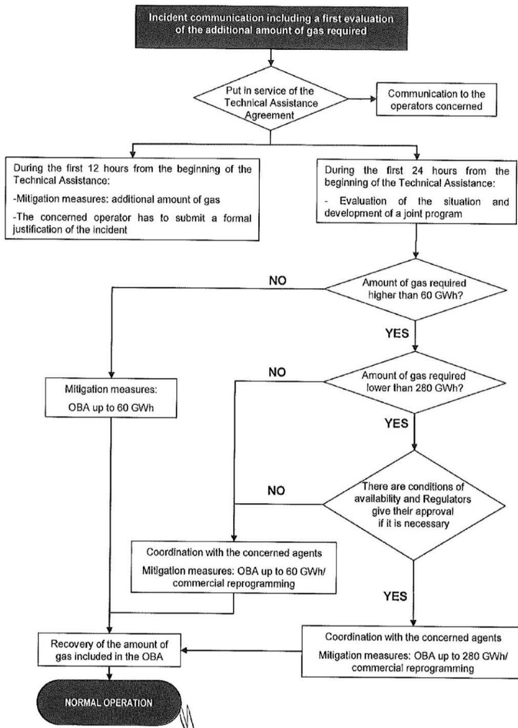
Figure X. Flowchart between Enagas and REN (VIP Iberico)
